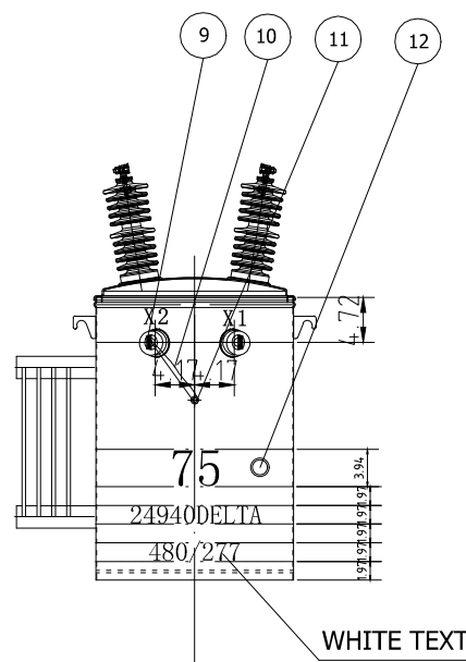
LV BUSHING TERMINAL
